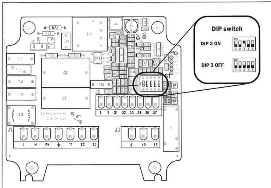
Fig. 2 DIP switch
