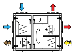
Supply air top
