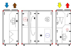
Size 17 h , 22 h and 28 with cooling unit
