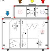
Sizes 04, 06 and 10 with cooling unit
