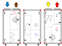
Sizes 09, 12, 17 and 22 with cooling unit
