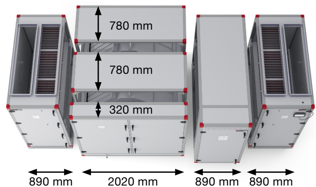
Envistar Top size 28 with EcoCooler and split counter-flow exchanger.
