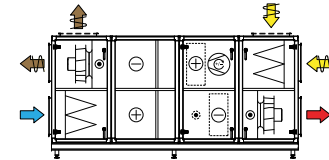
Comb. 12 Run-around coil unit and cooling unit
