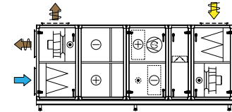
Comb. 14 Run-around coil unit, cooling unit, recirculating unit
