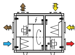
Supply air bottom
