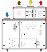
Sizes 04, 06 and 10 with cooling unit
