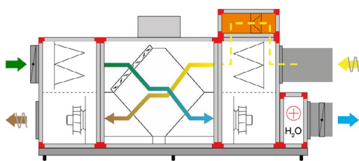
Integrated filter-bypass on the extract air
