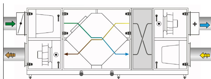
New installation, with cross-flow section
