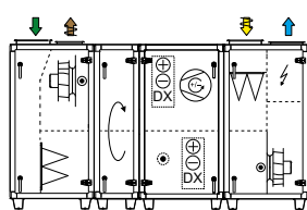
Rotor and reversible heat pump sizes 09, 12, 17 and 22
