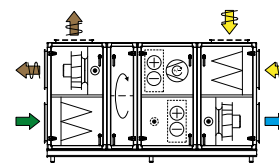
Rotor and reversible heat pump
