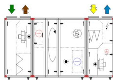
Size 17 h , 22 h and 28 with cooling unit
