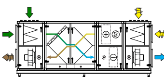
Comb. 8 Counter-flow heat exchanger and cooling unit
