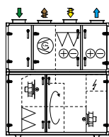
Rotor and reversible heat pump sizes 06 and 10
