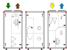
Sizes 09, 12, 17 i and 22 i with cooling unit
