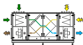
Comb. 7 Counter-flow heat exchanger
