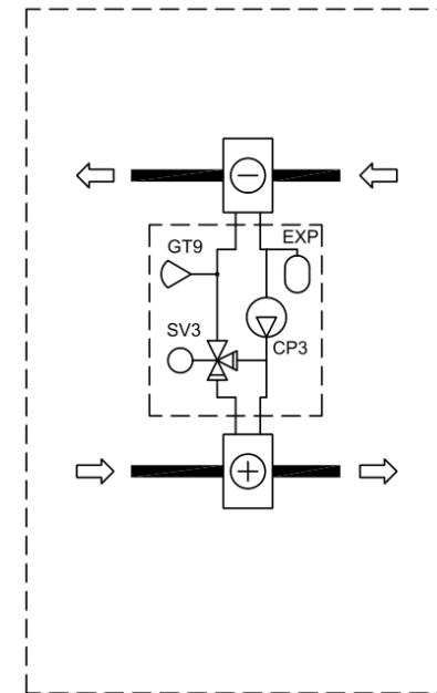
Coil heat exchanger (Run-around coil)
