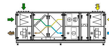
Comb. 10 Counter-flow heat exchanger, cooling unit, recirculating unit
