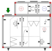
Sizes 04, 06 and 10 with cooling unit
