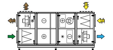
Comb. 12 Run-around coil unit and cooling unit
