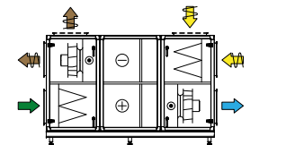
Comb. 11 Run-around coil unit
