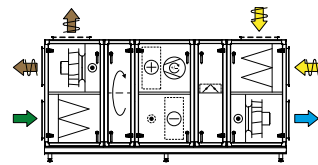
Comb. 5 Rotor, cooling unit and recirculating unit
