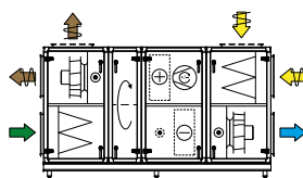
Comb. 2 Rotor and cooling unit
