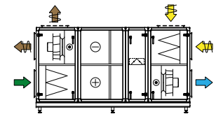
Comb. 13 Run-around coil unit and recirculating unit
