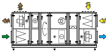
Comb. 6 Cooling unit with cooling recovery and recirculating unit
