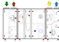
Size 17 h , 22 h and 28 with cooling unit
