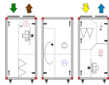
Sizes 09, 12, 17 i and 22 i with cooling unit
